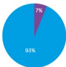
Compute Capacity
