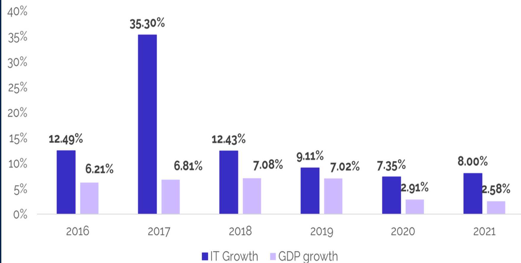
Vietnam IT Industry Growth & GDP Growth
